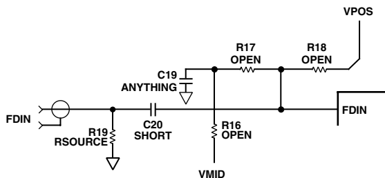
Figure 13. Evaluation Board
