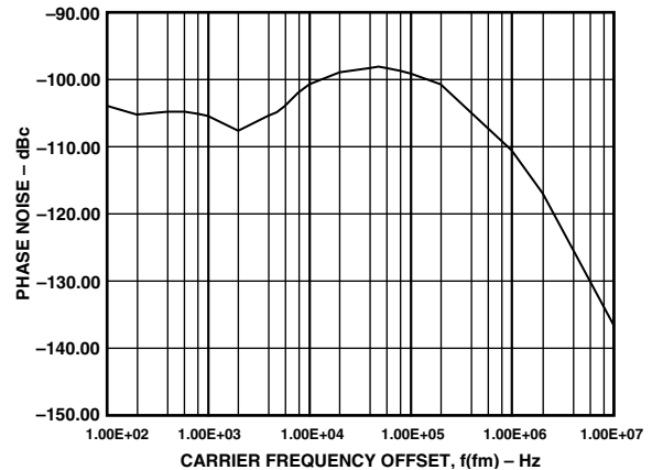
TPC 22. PLL Phase Noise L(F) vs. Frequency, V_{\text{POS}} = 3\text{ V} , C3 = 0.1\text{ }\mu\text{F} , \text{IF} = 10.7\text{ MHz}
