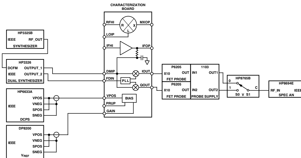
TPC 11. Quadrature Accuracy Test Set
