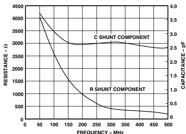
TPC 14. Mixer Input Impedance vs. Frequency, V_{\text{POS}} = 3\text{ V} , V_{\text{GAIN}} = 0.8\text{ V}
